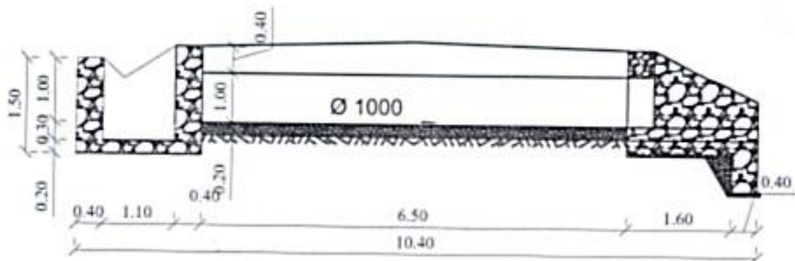
LONGITUDINAL CROSS-SECTION
